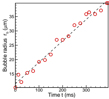
Bubble evolution during boiling
