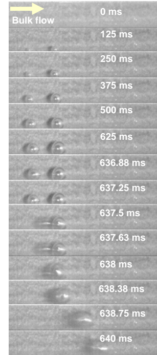
Twin bubbles agglomerate after growth and travel down the channel (8000 fps).
