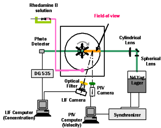
Fig. 1 Experimental Setup for PIV/LIF simultaneous measurement
