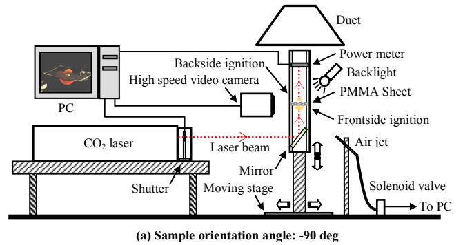
Experimental apparatus
